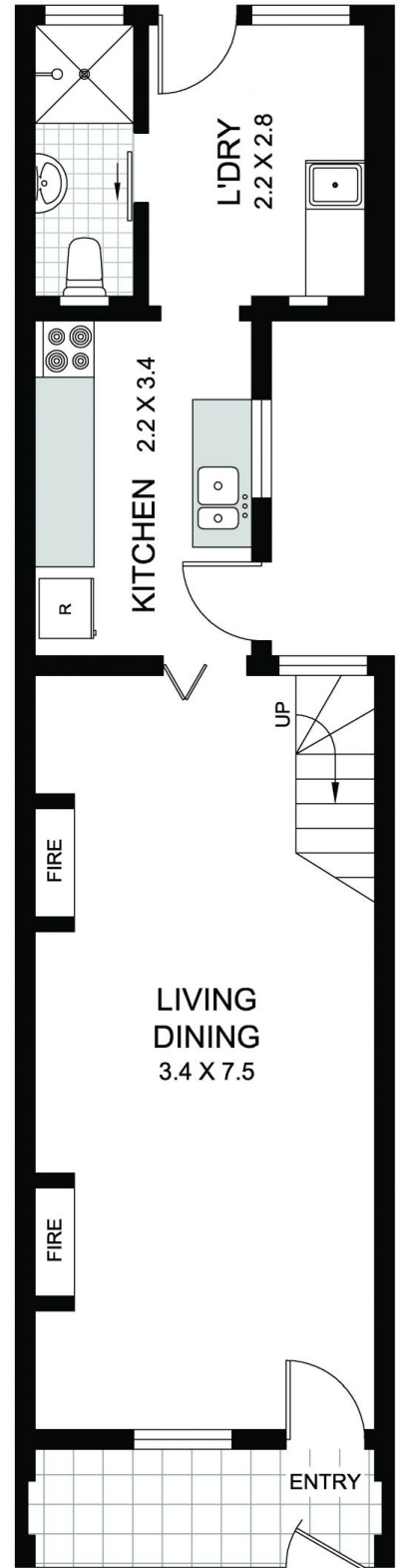
LEVEL 1
