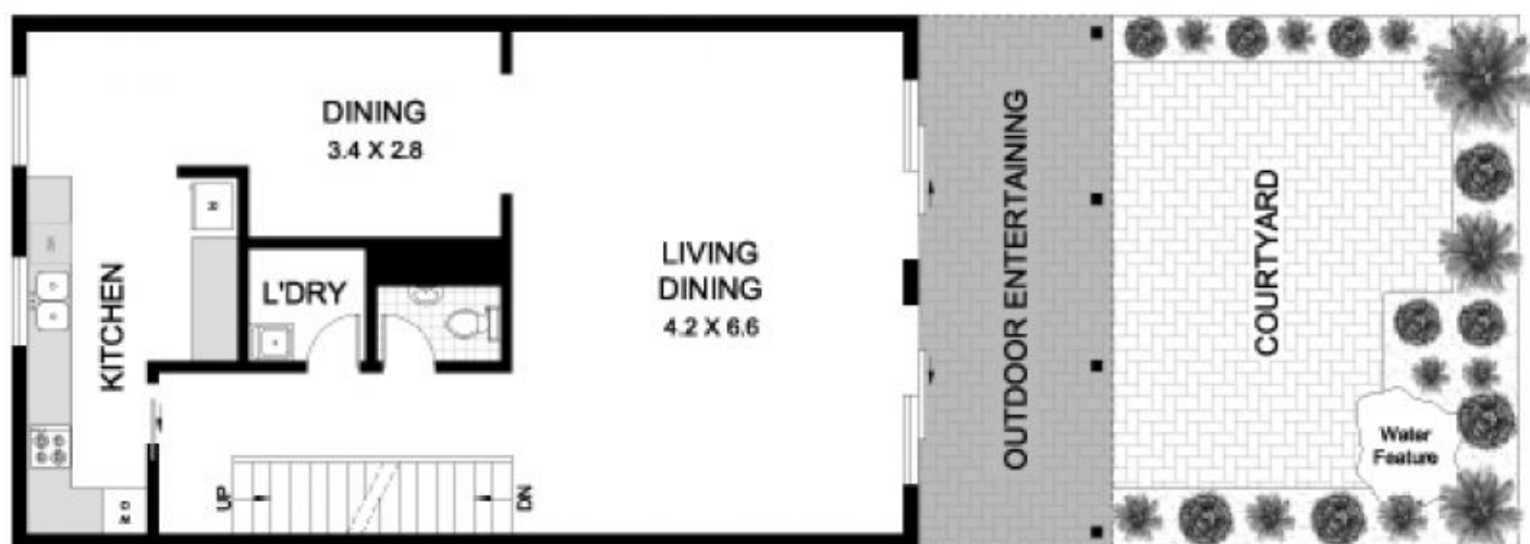
LEVEL 1
